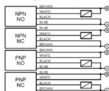
4 wires (NO+NC)
