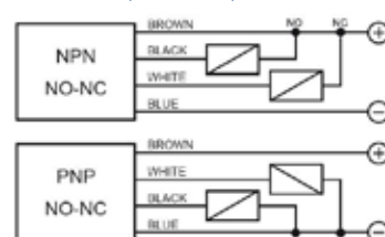
4 wires (NO+NC)
