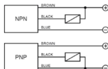
4 wires (PNP/NPN, NO/NC)
